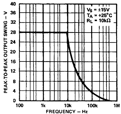
Figure 12. Output Voltage Swing vs. Frequency
