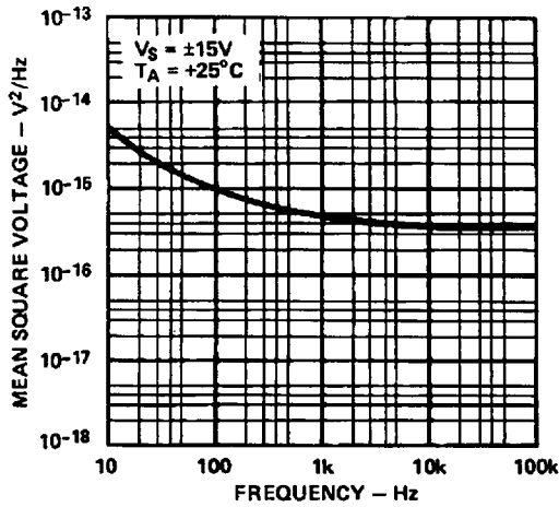
Figure 7. Input Noise Voltage vs. Frequency
