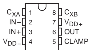
D014, J, OR N PACKAGE (TOP VIEW)
