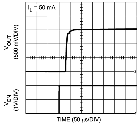
Enable Start Up Timing, ( V_{OUT} = 1.5\text{V} )
