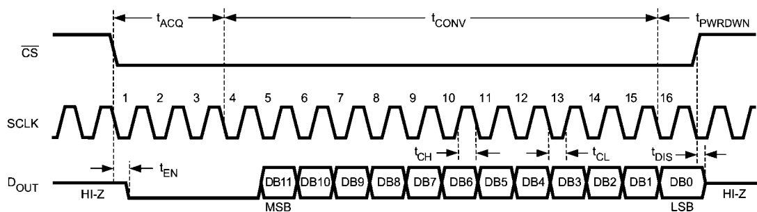
FIGURE 1. ADC121S705 Single Conversion Timing Diagram
