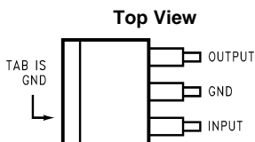
Figure 3. DDPAK/TO-263 Surface-Mount Package See Package Number KTT0003B
