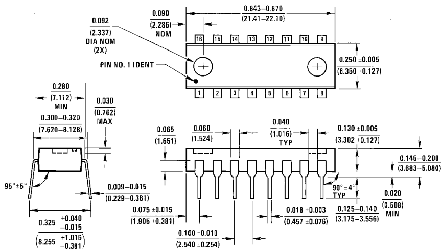
16-Pin Molded Dual-In-Line Package Order Number LMC6684AIN or LMC6684BIN NS Package Number N16A
