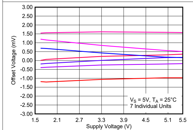
Figure 8-33. Offset Voltage vs. Supply Voltage, 25°C
