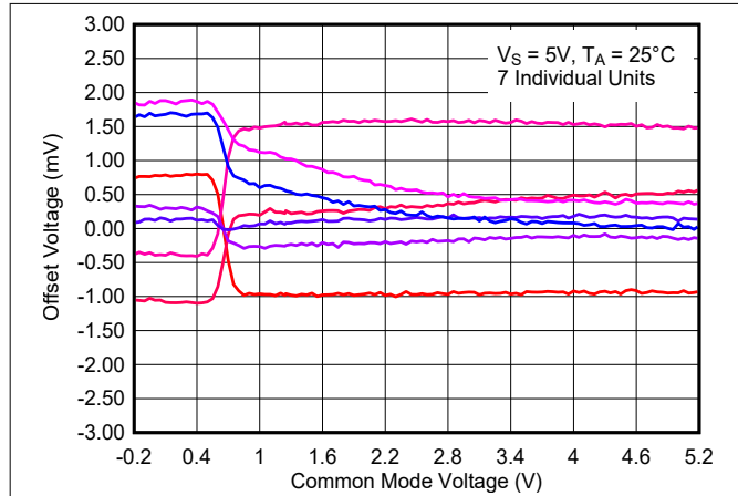
Figure 8-31. Offset Voltage vs. Common Mode Voltage, 5 V
