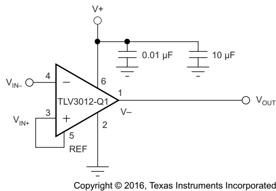
Figure 10-1. Basic Connections
