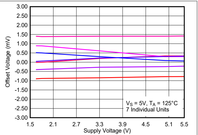
Figure 8-32. Offset Voltage vs. Supply Voltage, 125°C
