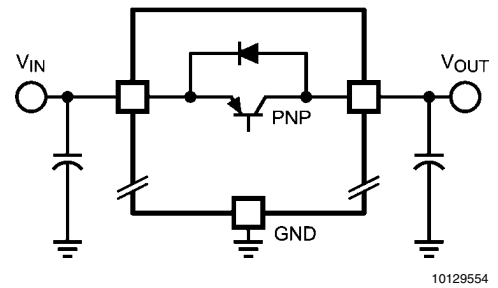
FIGURE 3. Reverse Current Path
