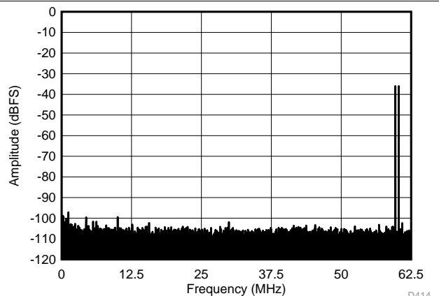
f_S = 125\text{ MSPS} , IMD = 97\text{ dBFS} , f_{IN1} = 185\text{ MHz} , f_{IN2} = 190\text{ MHz}
