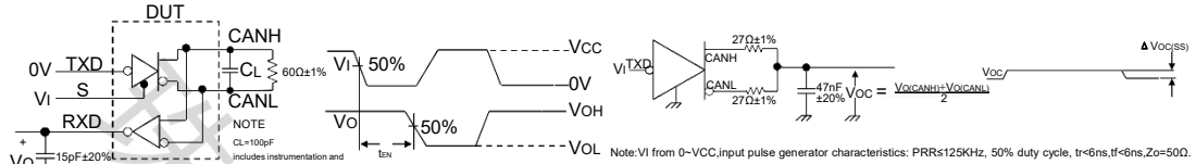
F8. Common Mode Output Voltage Test and
