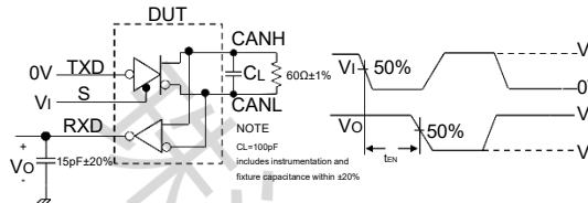
F7. t EN Test Circuit and Voltage Waveforms
