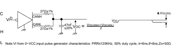
F8. Common Mode Output Voltage Test and Voltage Waveforms
