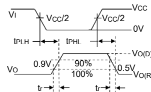
F4. Driver Test Circuit and Voltage Waveforms
