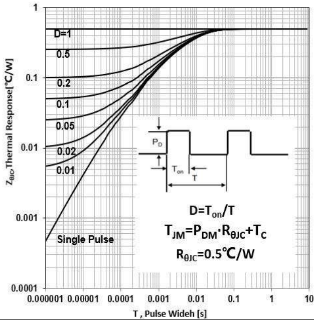
Figure 19. IGBT Transient Thermal Impedance vs Pulse Width(TO3PN/TO247)
