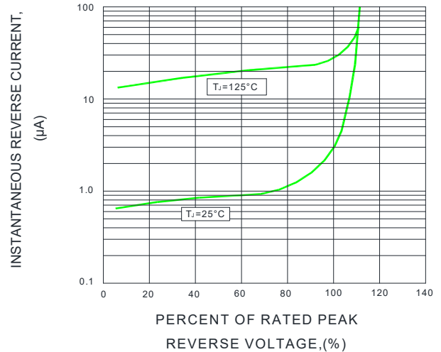
FIG.4-TYPICAL REVERSE CHARACTERISTICS
