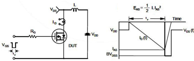
Fig14. Unclamped Inductive Test Circuit and waveforms
