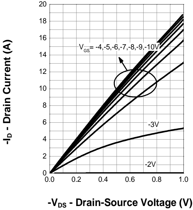
Output Characteristics
