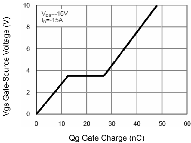
Figure 11 Gate Charge
