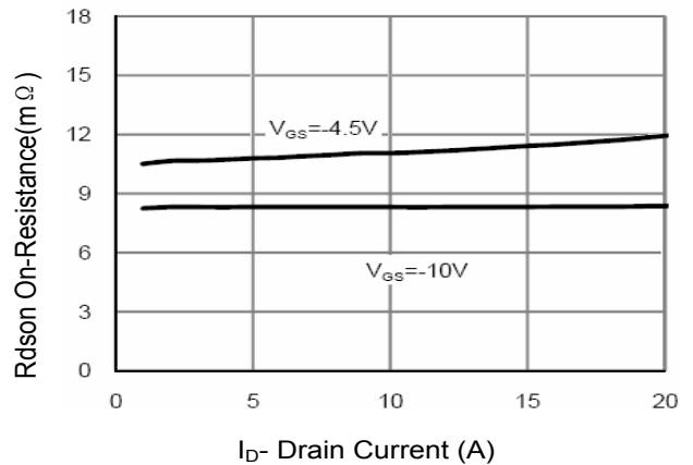
Figure 6 Drain-Source On-Resistance
