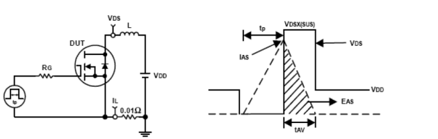
Fig10. Unclamped Inductive Test Circuit and waveforms
