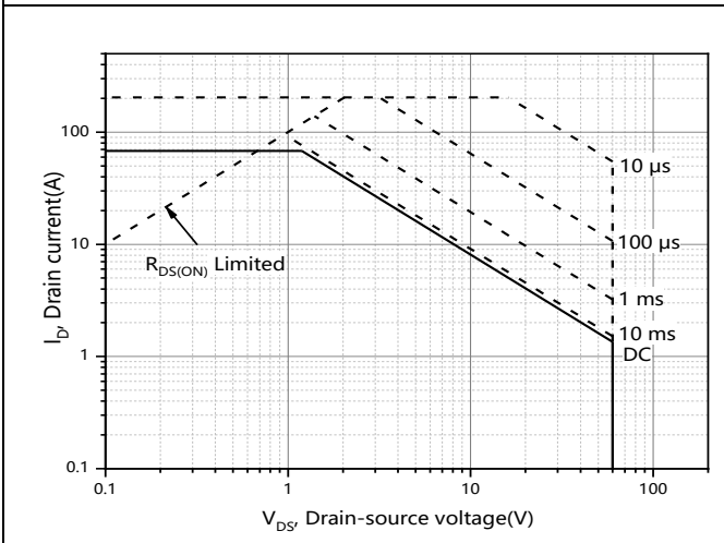
Figure 11. Safe operation area TC=25 °C
