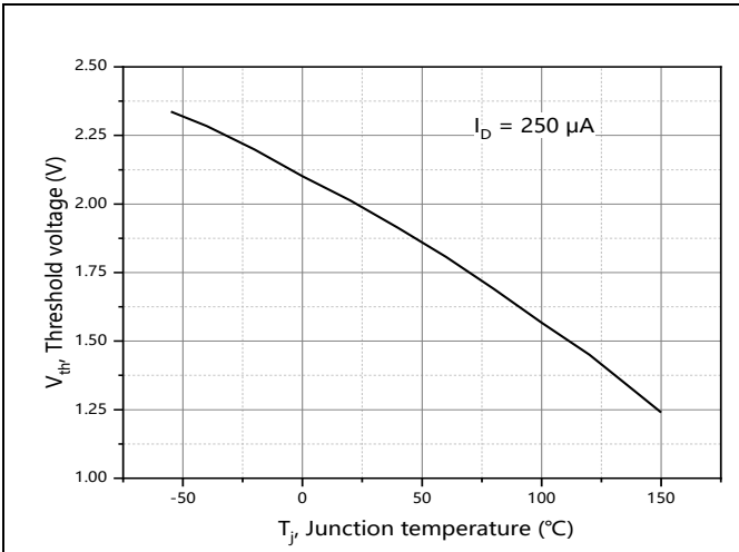
Figure 7. Threshold voltage
