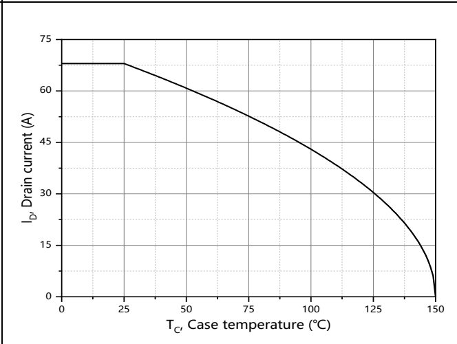
Figure 10. Drain current
