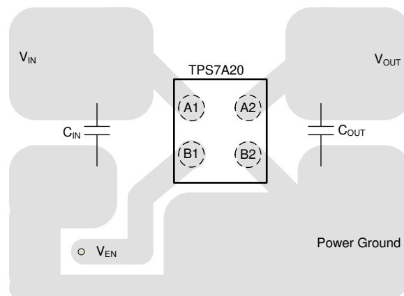
Figure 10-3. YCJ and YCK Package (DSBGA) Typical Layout
