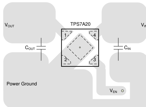
Figure 10-2. DQN Package (X2SON) Typical Layout
