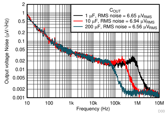
Figure 6-68. Noise vs Frequency and C_{OUT}
