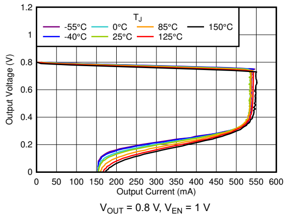
Figure 6-45. Current Limit
