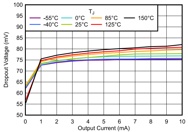
Figure 6-32. Dropout Voltage vs I_{OUT}
