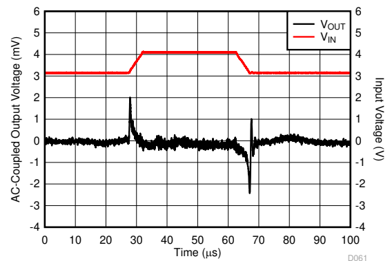
Figure 6-58. Load Transient
