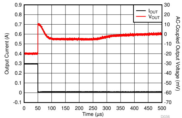
Figure 6-56. Load Transient
