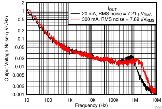
Figure 6-70. Noise vs Frequency and I_{OUT}
