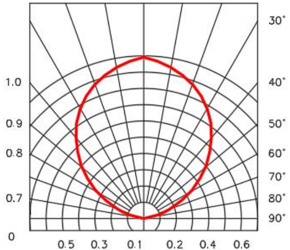
Radiation diagram 0° 10° 20°
