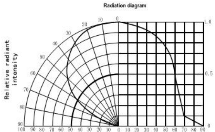
Fig.6 SPATIAL DISTRIBUTION
