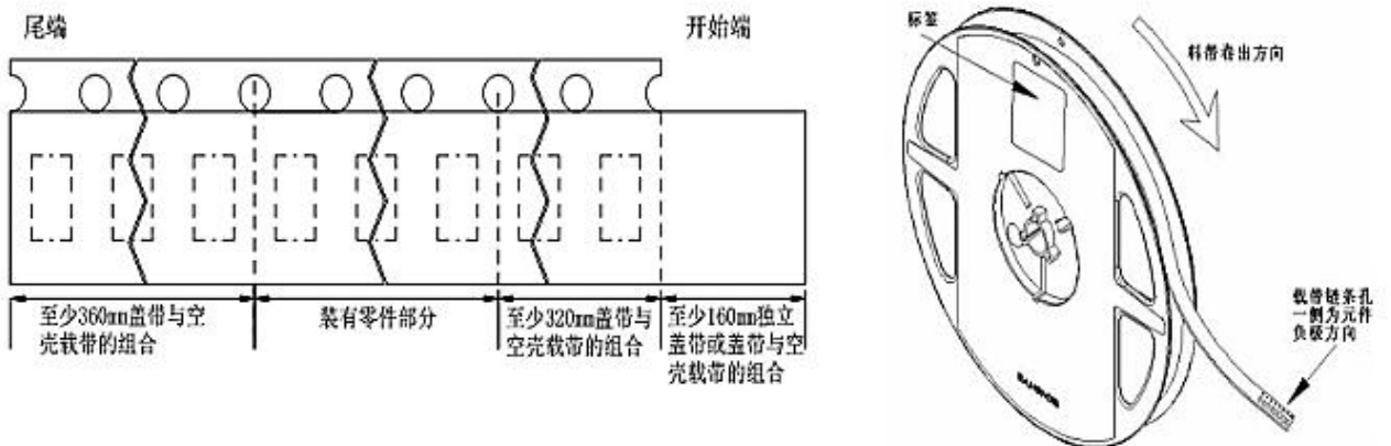
圆盘及载带卷出方向及空穴规格 Disk and carrier belt direction of roll and hole dimensions
