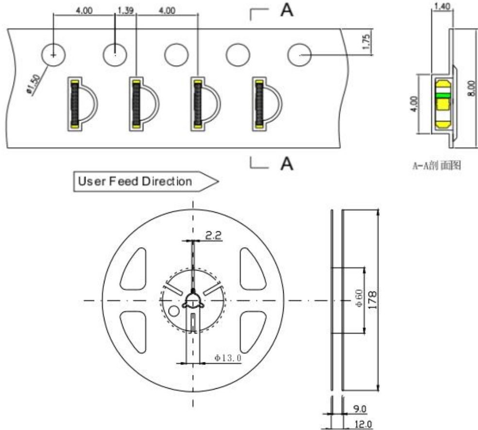
载带与圆盘尺寸 Belt and disk dimensions
