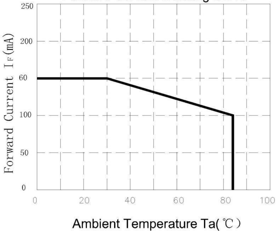
Forward Current Derating Curve
