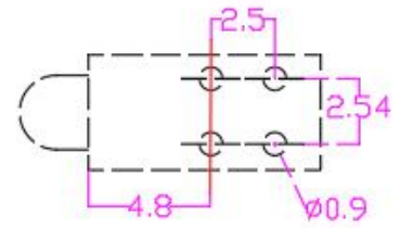
建议焊盘尺寸: Recommended Soldering Pattern
