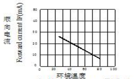
环境温度 Ambient Temperature T_A(^{\circ}C) Fig.3 Forward Current Derating Curve
