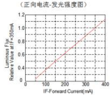
Forward current - luminous intensity curve (正向电流-发光强度图)
