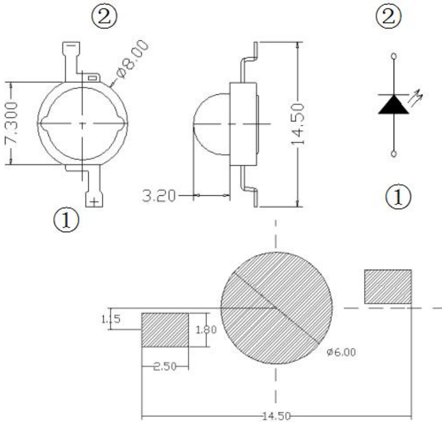
推荐焊盘 Recommand soldering pad
