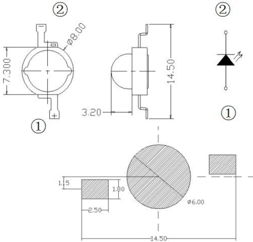
推荐焊盘 Recommant soldering pad
