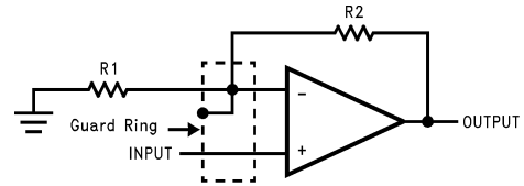
Non-Inverting Amplifier
