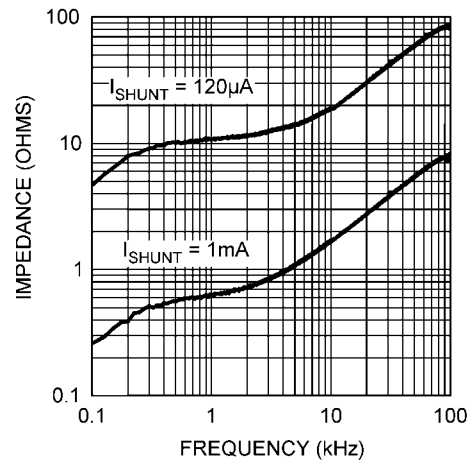
Reverse Dynamic Impedance vs Frequency
