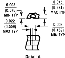
Ceramic Leadless Chip Carrier Package (E) Order Number 54LS20LMQB Package Number E20A
