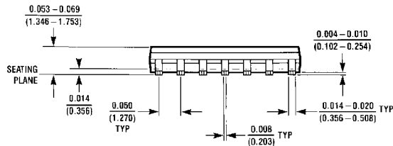
14-Lead Small Outline Molded Package (M) Order Number DM74LS20M Package Number M14A
