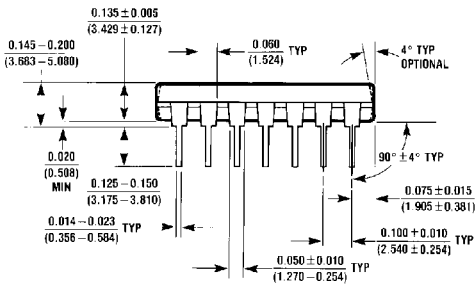
14-Lead Molded Dual-In-Line Package (N) Order Number DM74LS20N Package Number N14A
