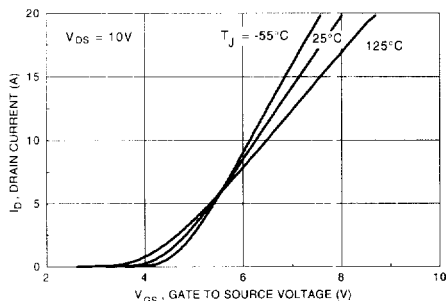
Figure 5. Transfer Characteristics.
