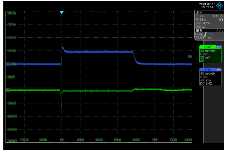
I_{OUT}: 0 \sim 40\text{mA}
