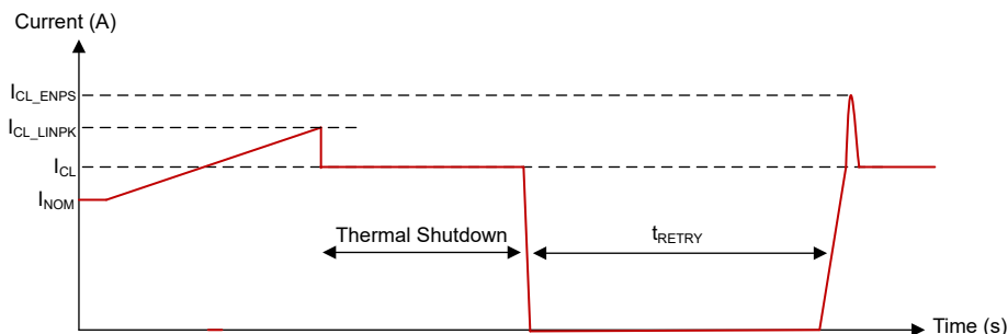
图 8-14. Overload Behavior
