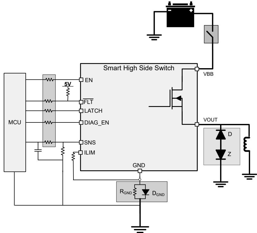
图 8-21. Loss of Battery
