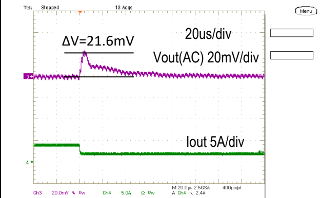
Step Load Transient Response (Vin=12V, Vout=1.0V, Cload=400uF, Iout=4A to 2A, 2.5A/us)
