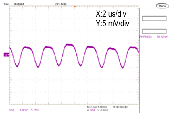
Output Ripple and Noise (Vin=12V, Vout=3.3V, Iout=4A, Cload=400uF, ScopeBW=20MHz)
