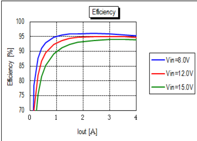
Efficiency vs. Line Voltage and Load Current @ +25degC. (Vout = 3.3V)
