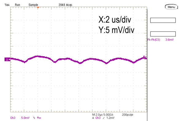
Output Ripple and Noise (Vin=5.0V, Vout=0.7V, Iout=4A, Cload=400uF, ScopeBW=20MHz)
