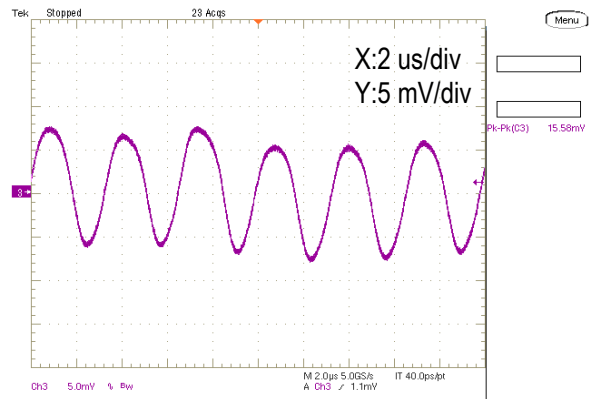
Output Ripple and Noise (Vin=12V, Vout=5.0V, Iout=4A, Cload=400uF, ScopeBW=20MHz)
