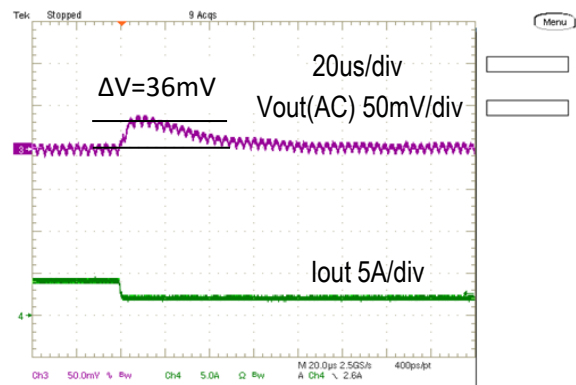
Step Load Transient Response (Vin=12V, Vout=3.3V, Cload=400uF, Iout=4A to 2A, 2.5A/us)
