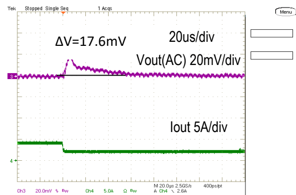
Step Load Transient Response (Vin=5.0V, Vout=1.0V, Cload=400uF, Iout=4A to 2A, 2.5A/us)
