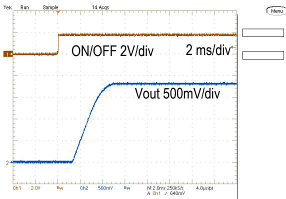
On/Off Enable Delay (Vin=5.0V, Vout=1.8V, Iout=4A, Cload=400uF)
