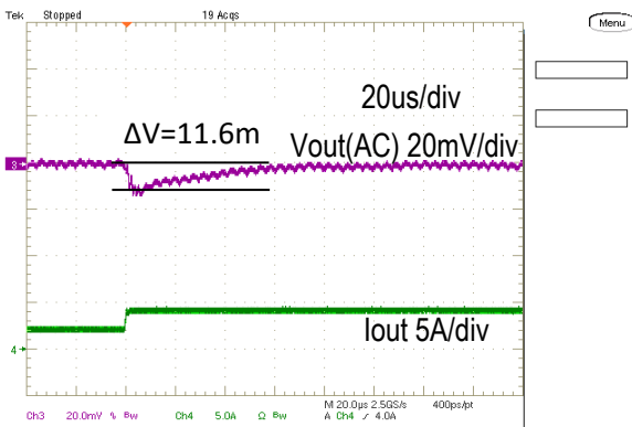
Step Load Transient Response (Vin=5.0V, Vout=1.0V, Cload=400uF, Iout=2A to 4A, 2.5A/us)
