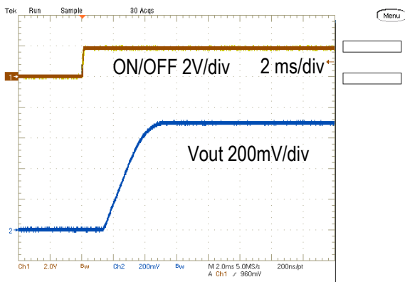
On/Off Enable Delay (Vin=5.0V, Vout=0.7V, Iout=4A, Cload=400uF)
