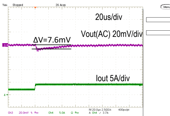
Step Load Transient Response (Vin=5.0V, Vout=0.7V, Cload=400uF, Iout=2A to 4A, 2.5A/us)
