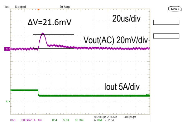
Step Load Transient Response (Vin=5.0V, Vout=0.7V, Cload=400uF, Iout=4A to 2A, 2.5A/us)
