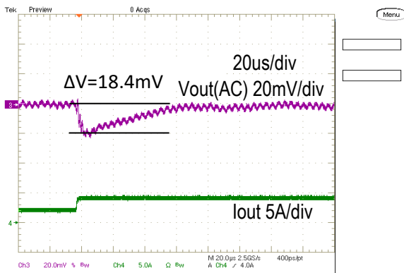
Step Load Transient Response (Vin=5.0V, Vout=1.8V, Cload=400uF, Iout=2A to 4A, 2.5A/us)
