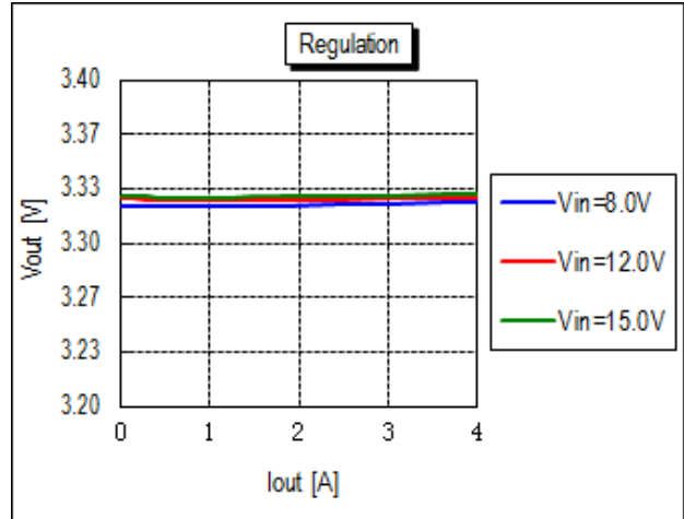
Vout vs. Line Voltage and Load Current @ +25degC. (Vout = 3.3V)
