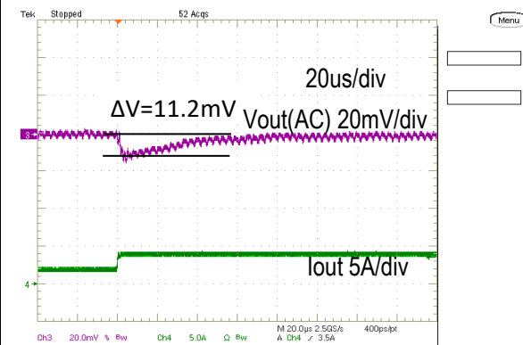
Step Load Transient Response (Vin=12V, Vout=1.0V, Cload=400uF, Iout=2A to 4A, 2.5A/us)
