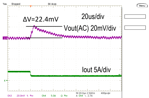
Step Load Transient Response (Vin=5.0V, Vout=1.8V, Cload=400uF, Iout=4A to 2A, 2.5A/us)
