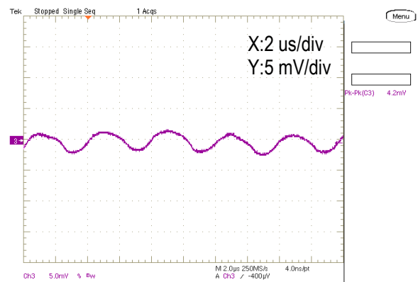
Output Ripple and Noise (Vin=5.0V, Vout=1.8V, Iout=4A, Cload=400uF, ScopeBW=20MHz)
