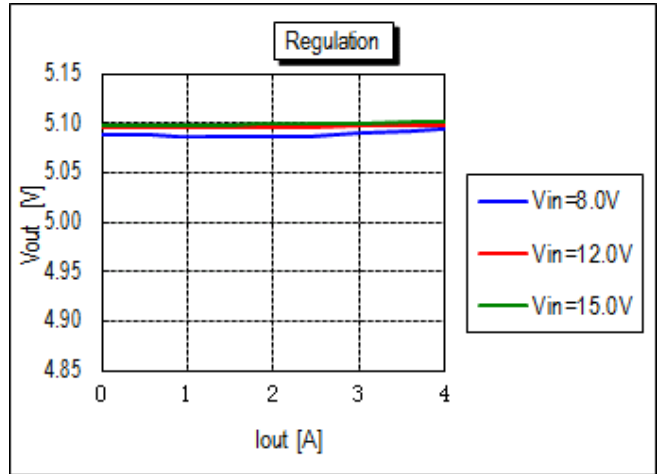
Vout vs. Line Voltage and Load Current @ +25degC. (Vout = 5.0V)
