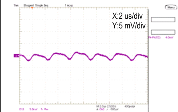
Output Ripple and Noise (Vin=12V, Vout=1.0V, Iout=4A, Cload=400uF, ScopeBW=20MHz)
