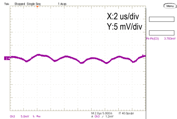
Output Ripple and Noise (Vin=5.0V, Vout=1.0V, Iout=4A, Cload=400uF, ScopeBW=20MHz)
