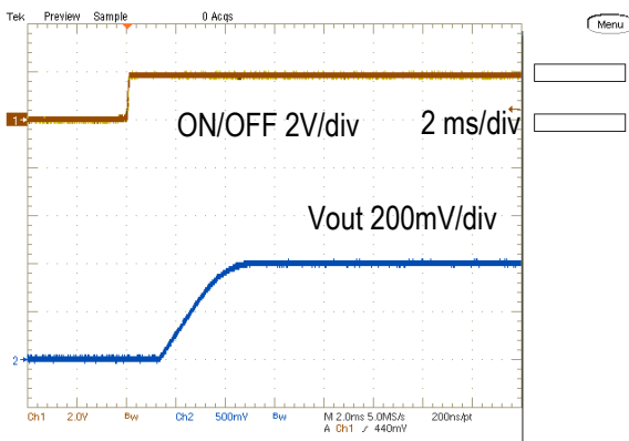
On/Off Enable Delay (Vin=5.0V, Vout=1.0V, Iout=4A, Cload=400uF)
