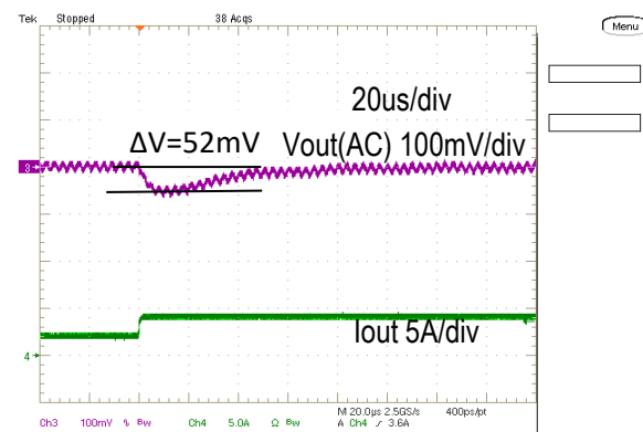
Step Load Transient Response (Vin=12V, Vout=5.0V, Cload=400uF, Iout=2A to 4A, 2.5A/us)
