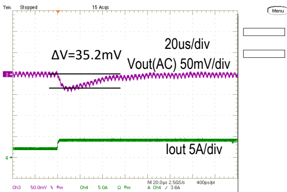
Step Load Transient Response (Vin=12V, Vout=3.3V, Cload=400uF, Iout=2A to 4A, 2.5A/us)
