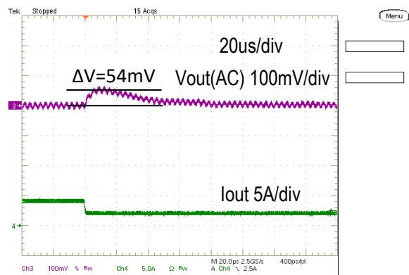
Step Load Transient Response (Vin=12V, Vout=5.0V, Cload=400uF, Iout=4A to 2A, 2.5A/us)
