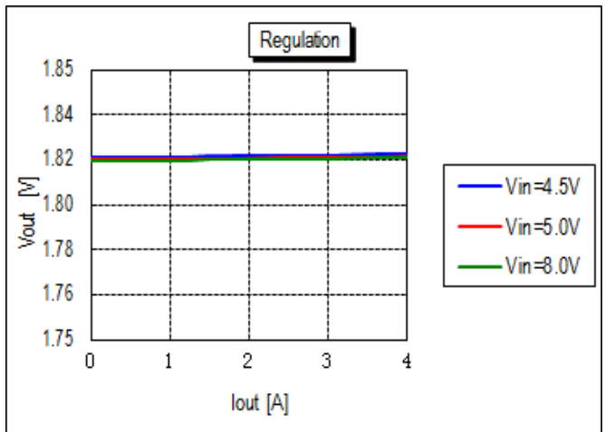
Vout vs. Line Voltage and Load Current @ +25degC. (Vout = 1.8V)
