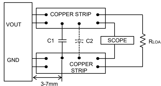
C1=220uF x 2 or 100uF x 4 CERAMIC C2=OPEN Figure: Measuring Output Ripple and Noise
