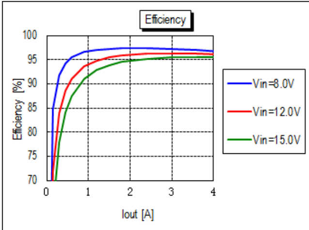
Efficiency vs. Line Voltage and Load Current @ +25degC. (Vout = 5.0V)
