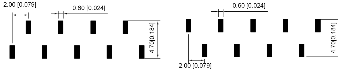
Recommended P.C.B Layout(Top Side) (PCB BOARD TOLERANCE±0.05)
