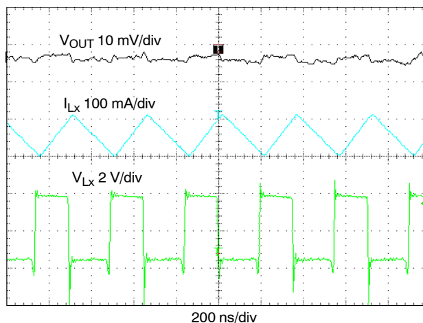
Figure 27. PWM Switching Waveform ( V_{IN} = 3.6\text{ V} , V_{OUT} = 1.2\text{ V} , I_{OUT} = 600\text{ mA} )
