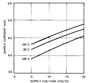
SUPPLY CURRENT vs SUPPLY VOLTAGE (OP-16/OP-17)
