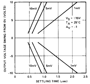
SETTLING TIME
