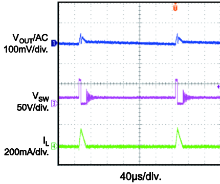
Steady State I_{OUT} = 5mA
