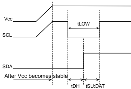
Figure 51. SCL='H' and SDA='L'
