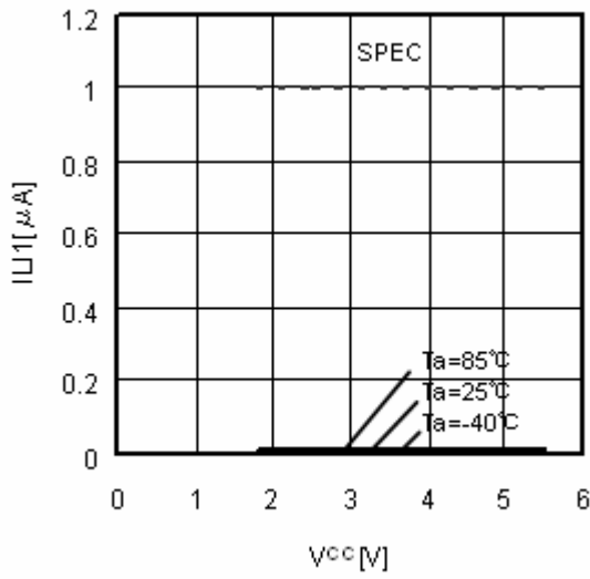
Figure 6. Input Leakage Current ILI1 (A0,A1,A2,SCL,SDA)
