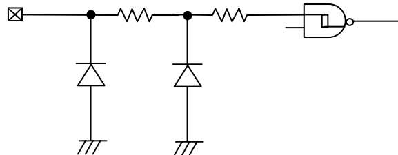
Figure 48. Input Pin Circuit
