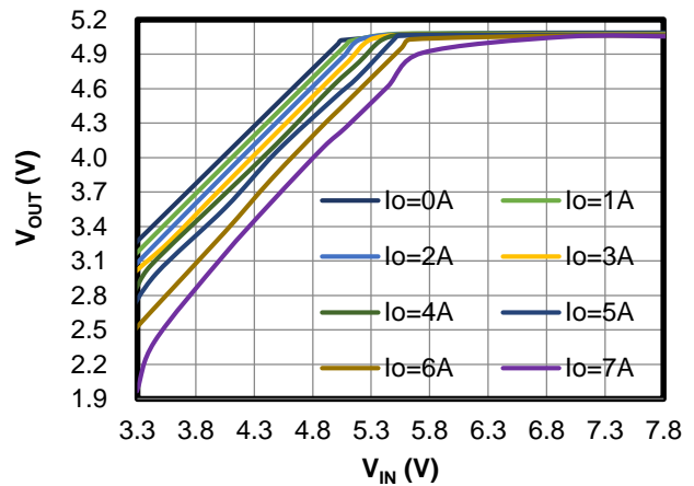
Low-Dropout Mode
