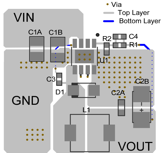
Figure 3: Recommended Layout
