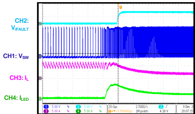
LED+ Short to GND Recovery
