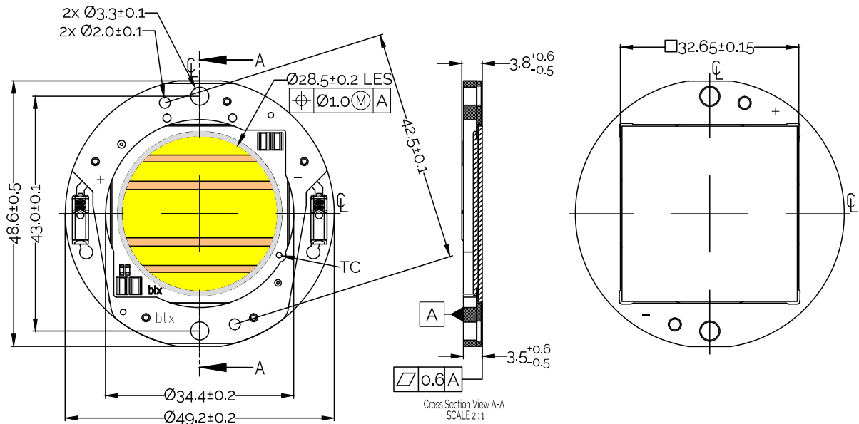
Figure 12: Mechanical Drawing Specifications
