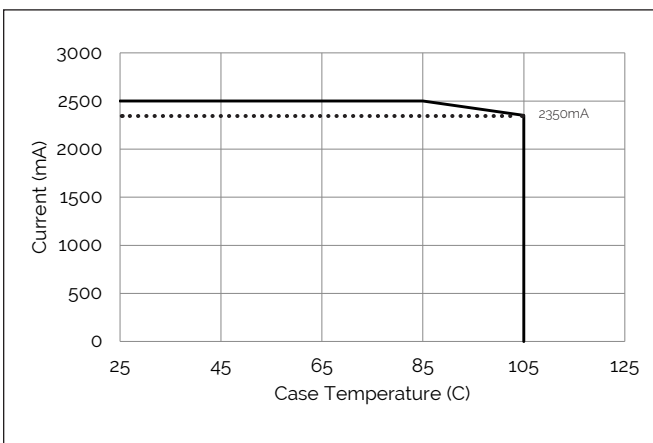
Figure 8: Derating Curve
