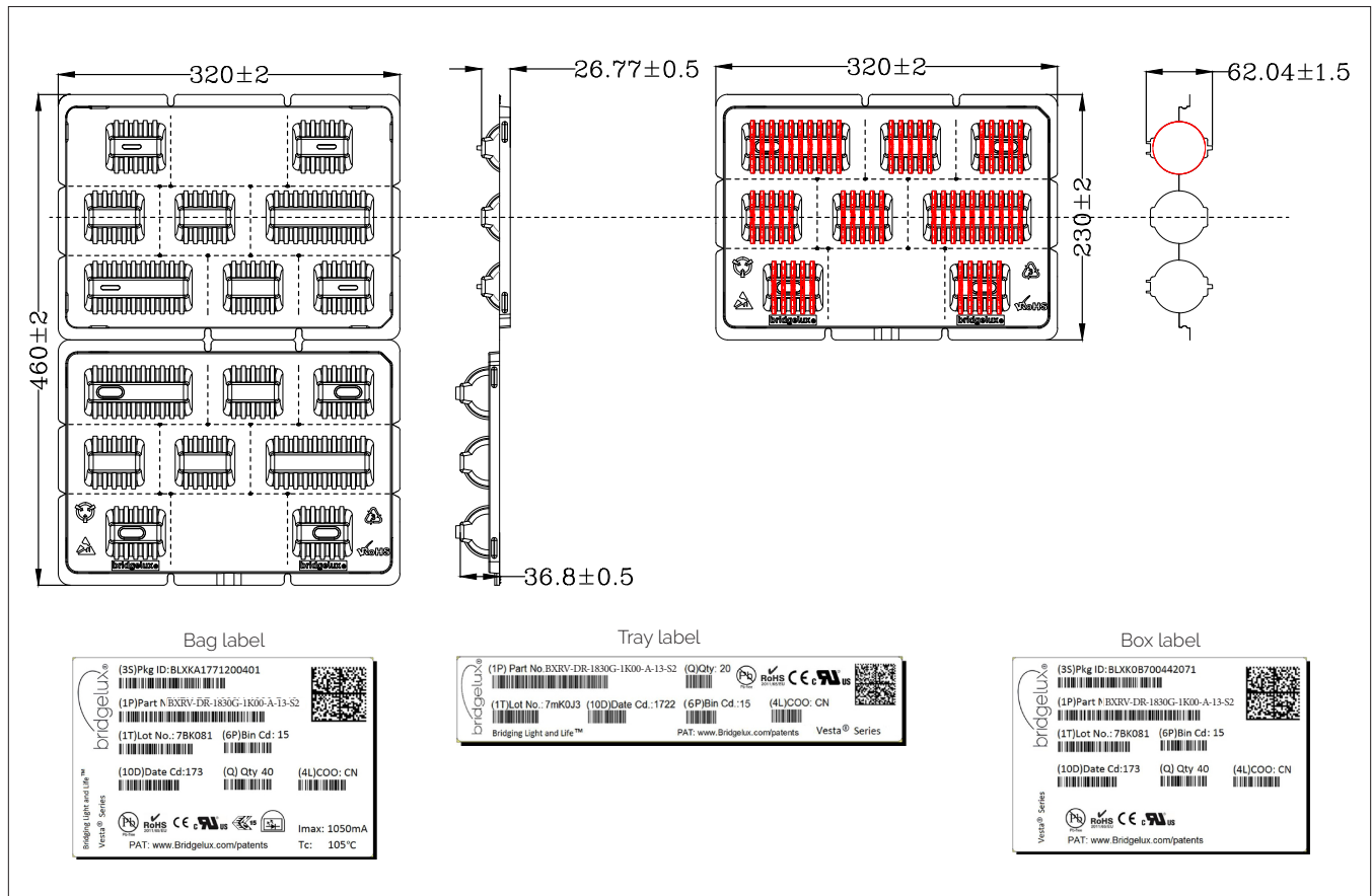
Figure 15: Packaging Specifications
