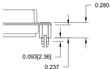
92X ..... 0.237" (BOARD SIDE)
