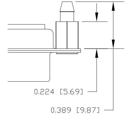
5 ..... 0.224" PCB SIDE
