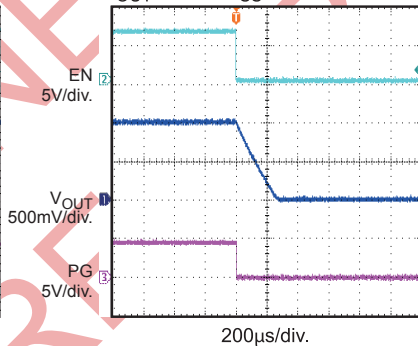
Power Good through EN Shutown
