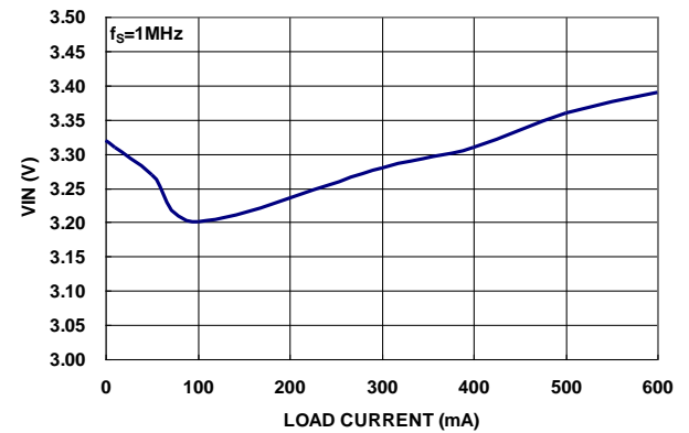
(a) V_{OUT}=3.3V
