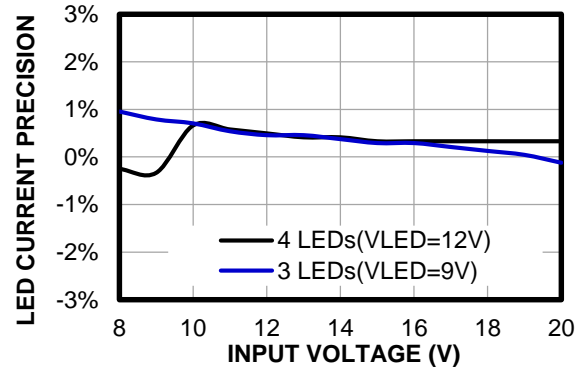
I_{LED} Precision vs. Input Voltage
